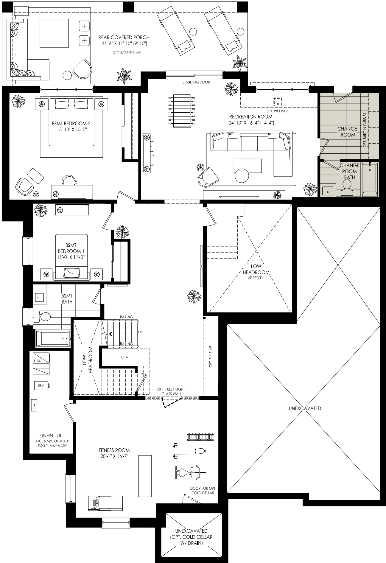
OPTIONAL FINISHED BASEMENT FLOOR PLAN W/ POOL CHANGE ROOM ELEV. 'A'
