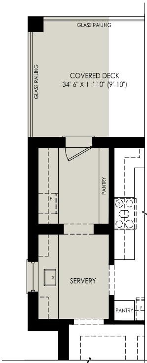
PARTIAL GROUND FLOOR PLAN OPTIONAL SERVERY DECK ACCESS ELEV. 'A'
