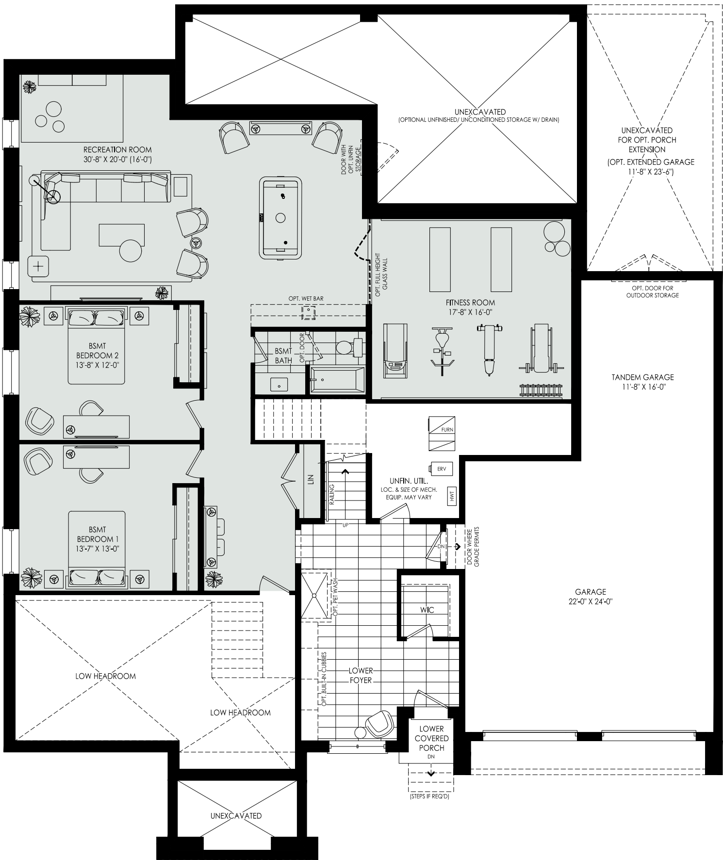
OPTIONAL FINISHED BASEMENT FLOOR PLAN ELEV. 'A'
