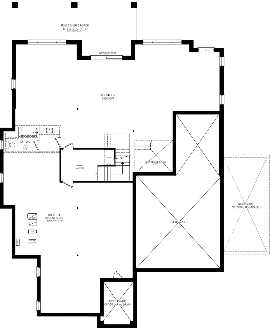
BASEMENT FLOOR PLAN ELEV. 'A'
